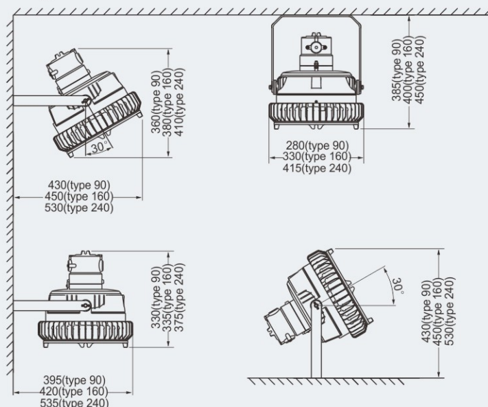
Bracket mounting dimension of type 90, type 160
