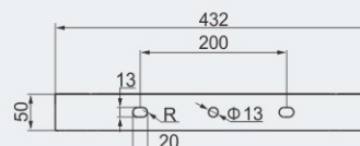
Bracket mounting dimension of type 240
