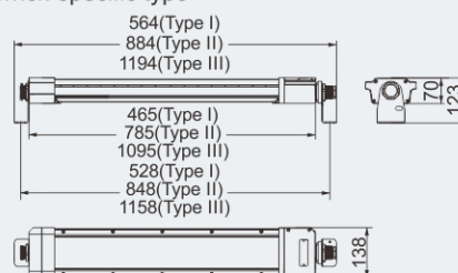
QT: derrick-specific type
